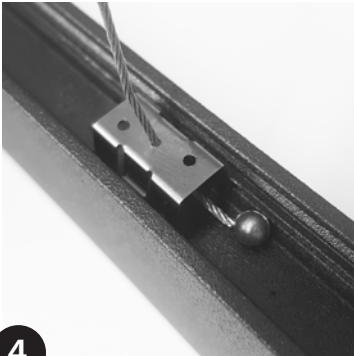
Correct Assembly.
